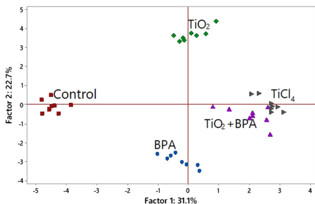
Fig. 5 Results of the principal component analysis of the studied biological traits of U. tumidus exposed to \text{TiCl}_4 (Ti), n- \text{TiO}_2 , BPA and n- \text{TiO}_2 + BPA for 14 days in comparison with the control (C) in the plane of two first principal components (Factors 1 and 2)
