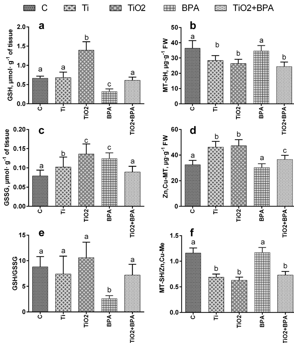
Fig. 2 Glutathione and metallothionein concentrations in the digestive gland of Unio tumidus exposed to TiCl_4 (Ti), n-TiO 2 , BPA and n-TiO 2 + BPA for 14 days, in comparison with the control (C). Data for a GSH; b metallothionein protein (MT-SH); c GSSG; d metalated metallothionein (Zn,Cu-MT); e GSH/GSSG ratio, f MT-SH/Zn, Cu-MT ratio of means, presented as mean \pm SD ( N = 8 for all indices except Zn,Cu-MT, N = 3 for Zn,Cu-MT sampled from 5 specimens in the group). If the letters above the bars are the same, this indicates that the values do not differ significantly ( P > 0.05 )
